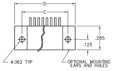
Plug
